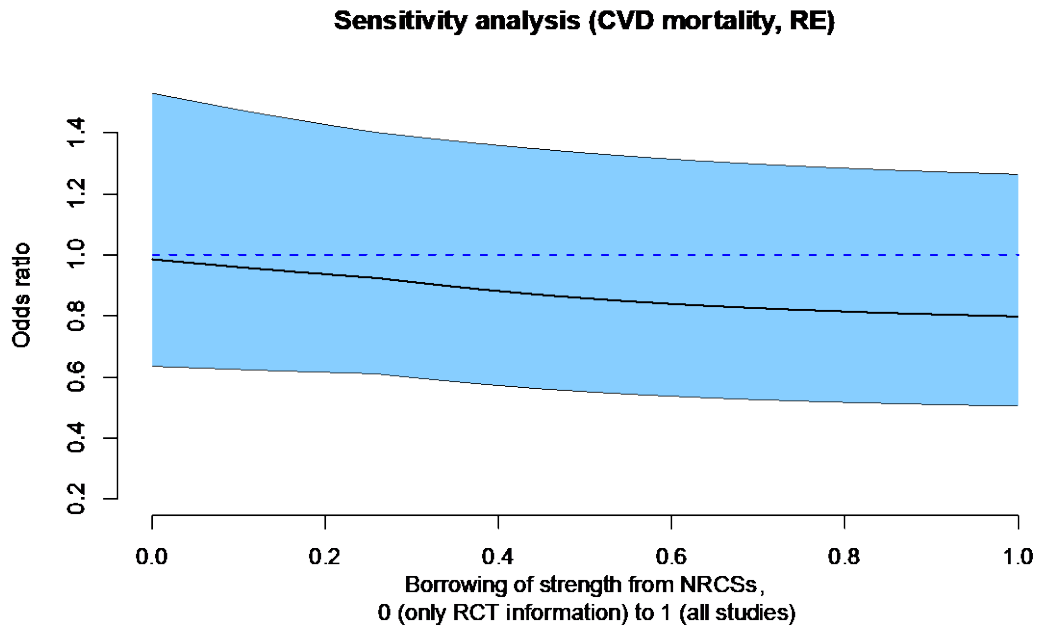
Figure D-3. Sensitivity Analysis: CVD Mortality
